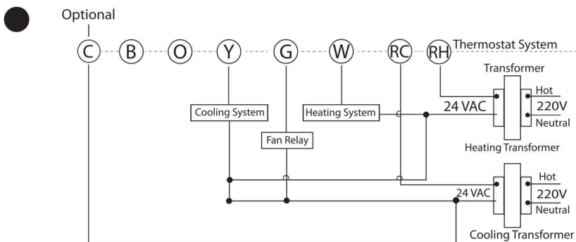
Typical Wiring Diagram For Heat/cool, 5 Wire, Two Transformer Systems
