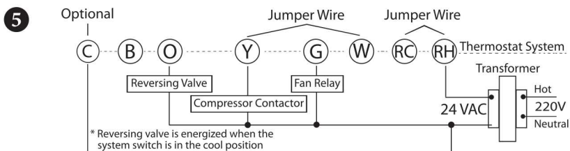
Typical Wiring Diagram For Heat Pump With Reversing Valve Energized In Cool
