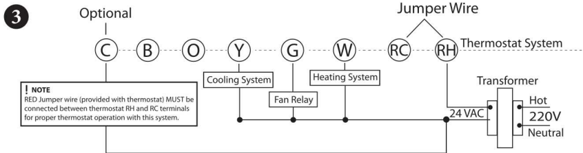
Typical Wiring Diagram For Heat/cool, 4 Wire, Single Transformer Systems
