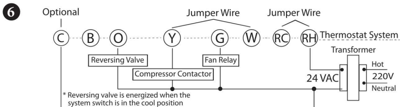
Typical Wiring Diagram For Heat Pump With Reversing Valve Energized In Heat
